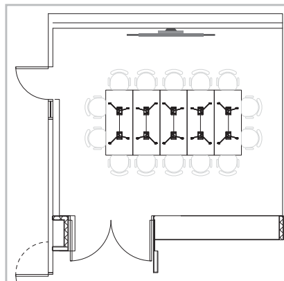
Layout 1: Boardroom, seats 14
